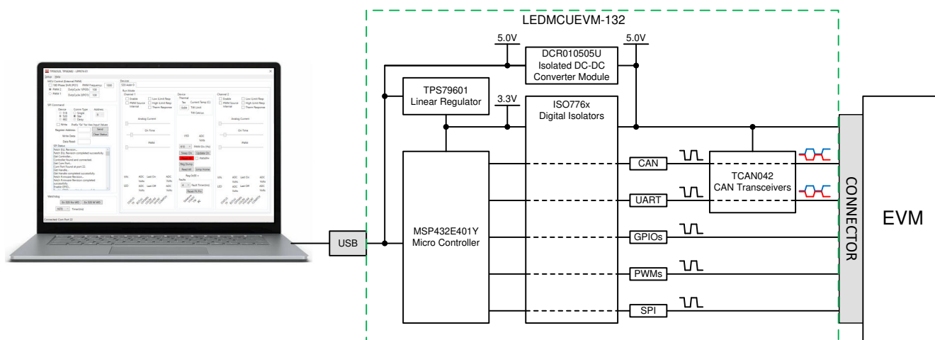
Figure 2-1. High-Level Diagram of the LEDMCUEVM-132
