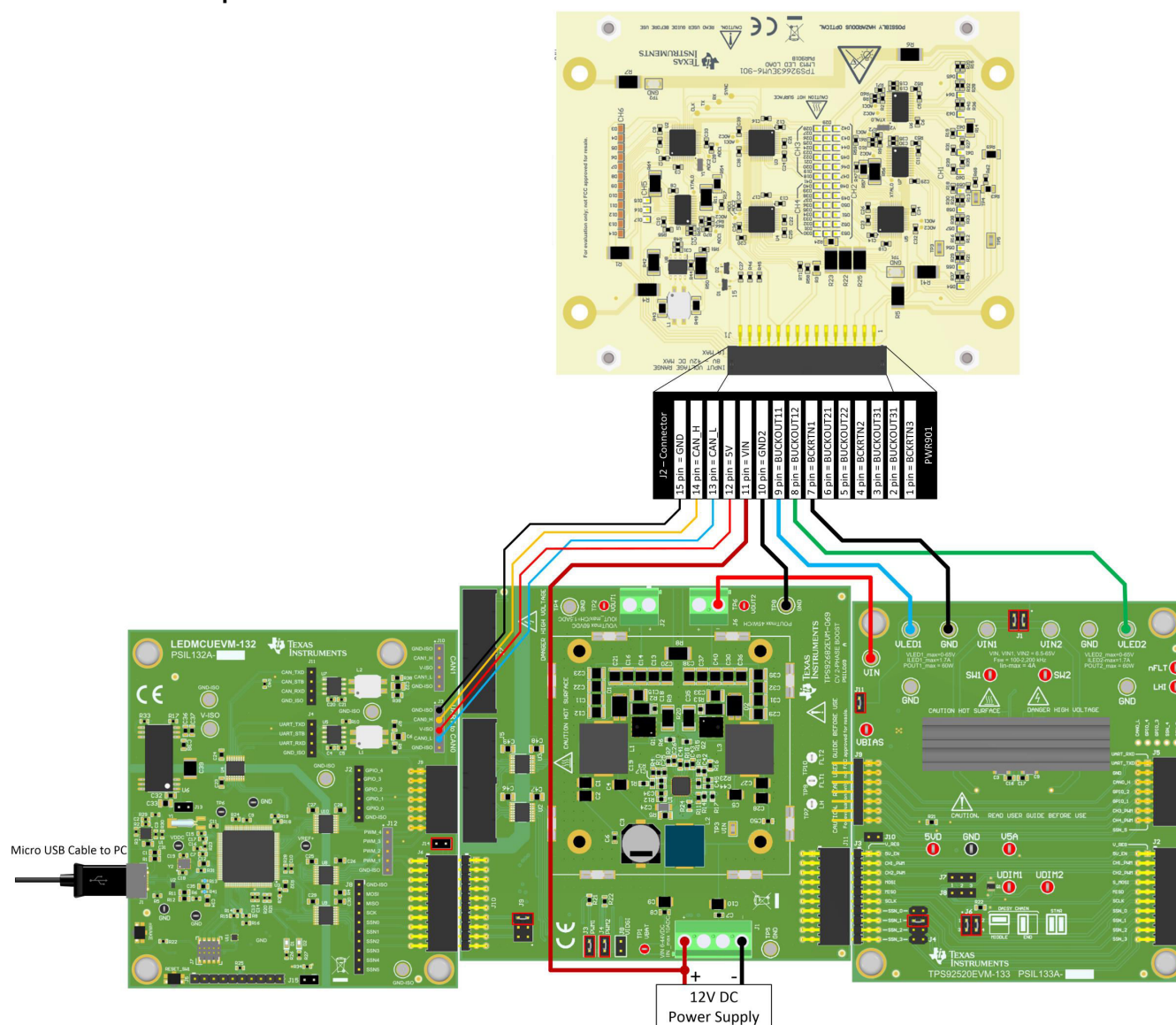
Figure 5-20. LEDMCUEVM-132 + TPS92682EVM-069 + TPS92520EVM-133 + TPS92662EVM6-901 Connections and Setup
